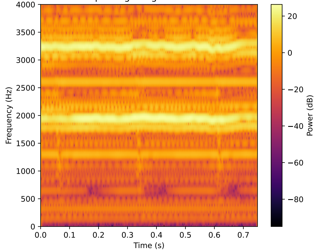
Spectrogram ground truth
