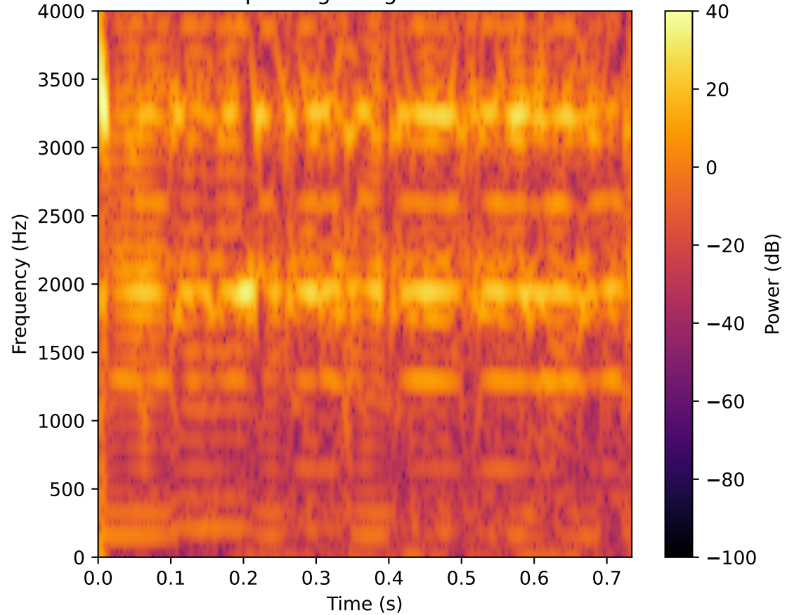
Spectrogram generated
